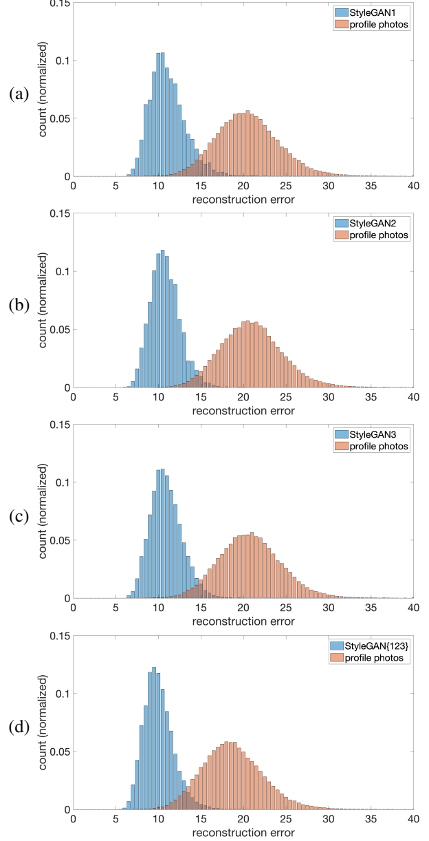
Figure 5. Normalized distributions of image reconstruction error from a learned latent embedding (autoencoder) (a-c) trained and evaluated separately on three versions of StyleGAN and real profile photos and (d) trained and evaluated on a combination of all three StyleGAN images.
